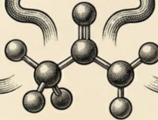
GLYCINE
